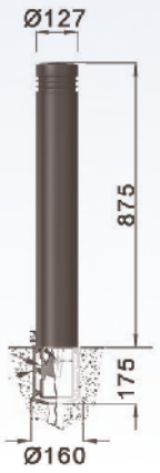
Borne amovible
